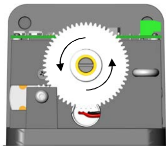
Anti-clockwise turning of the large gear will extend the bolt pin.
